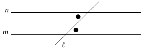
Figure 4.1: alternate interior angles
