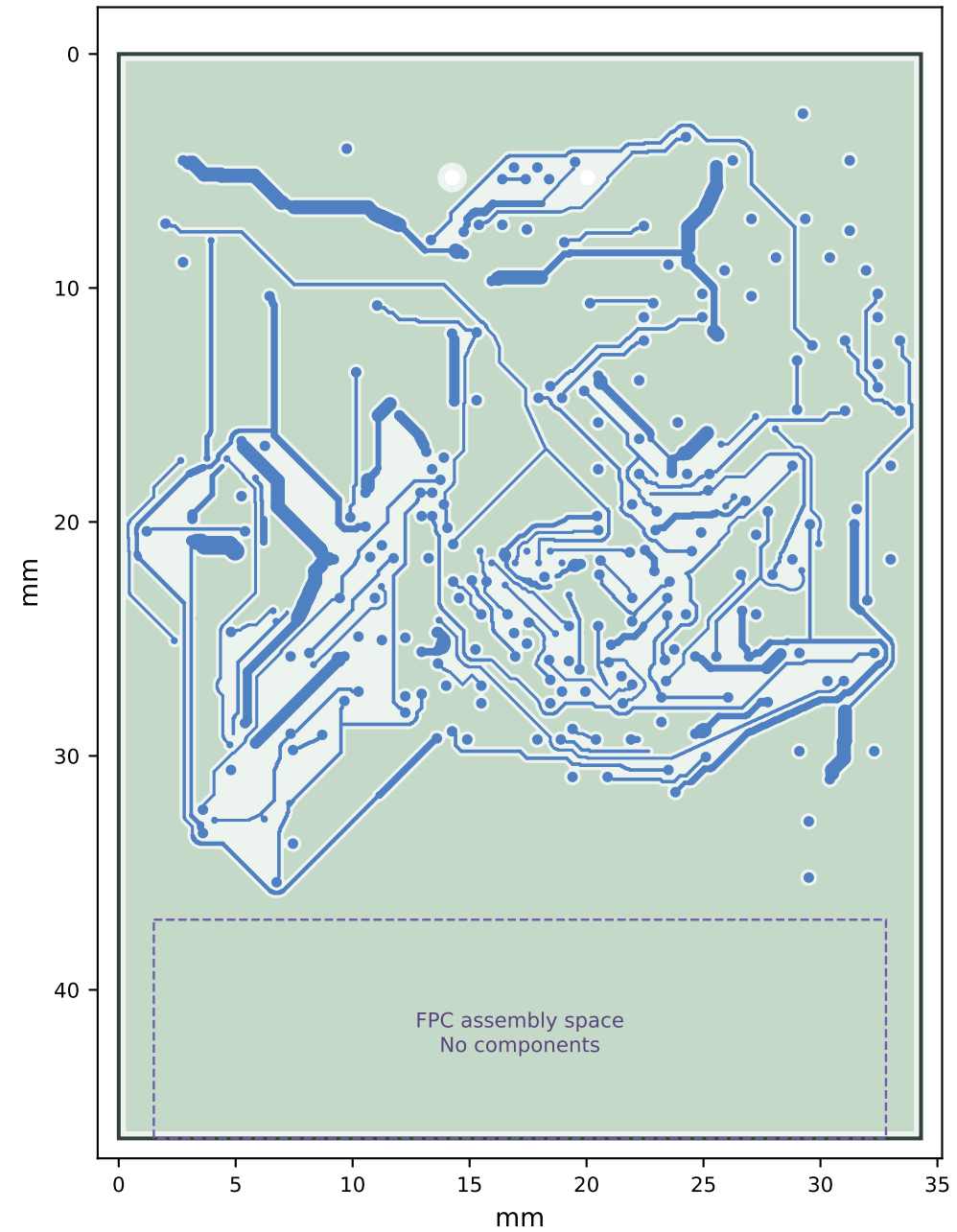
Bottom copper (through-board view)
