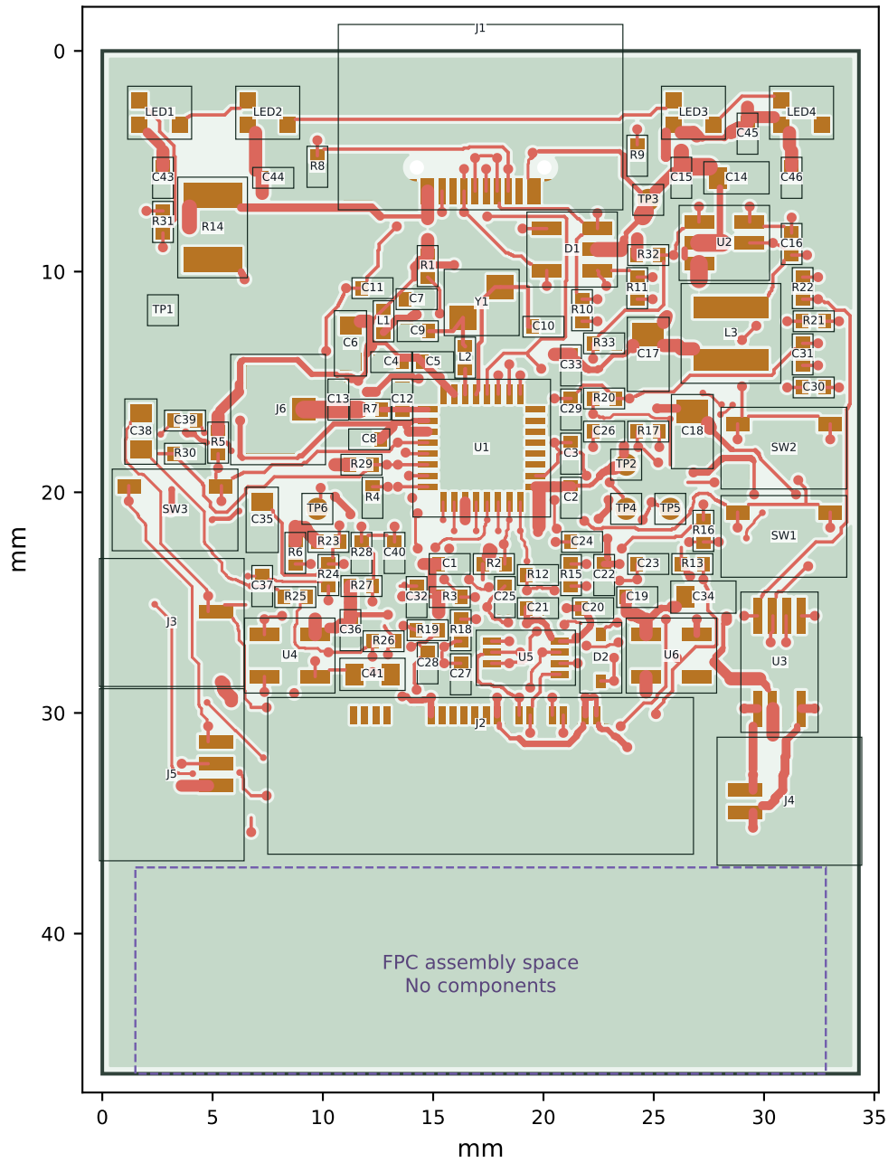
Top: components + copper
