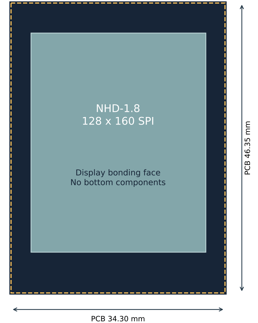
Screen / PCB envelope
