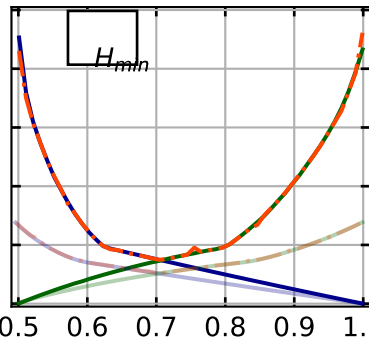
Optimal state discrimination
