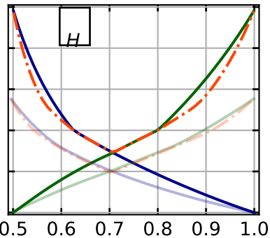
Optimal state discrimination
