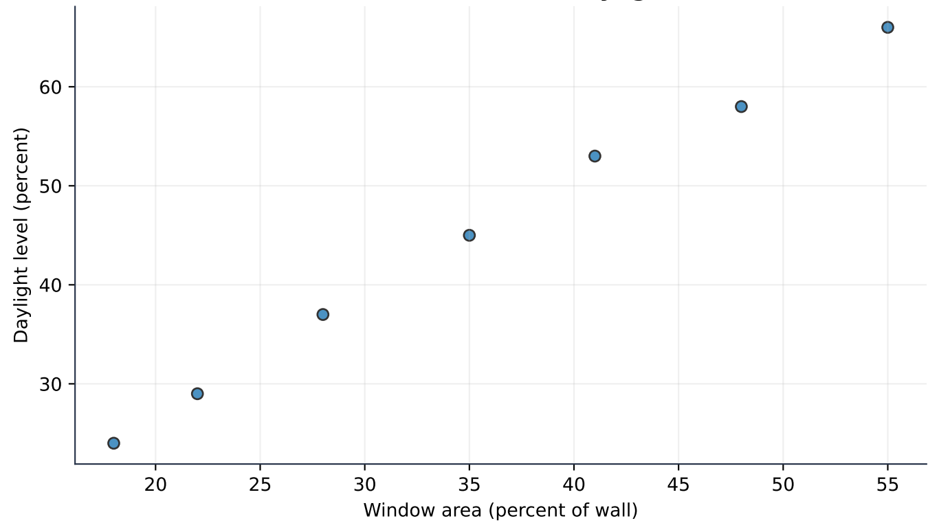
Window area and daylight
