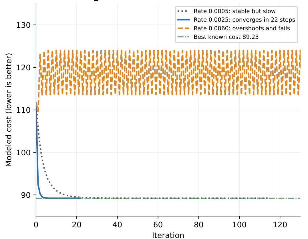
The learning rate decides whether descent works
