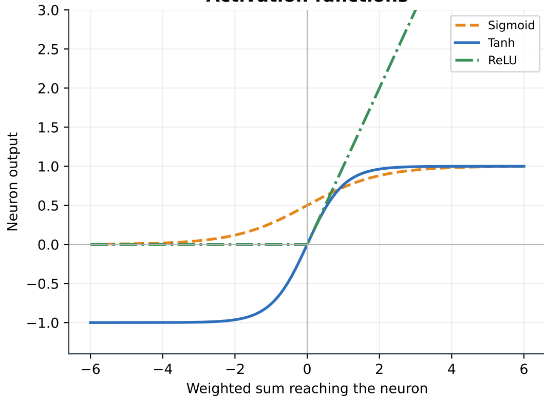
Activation functions
