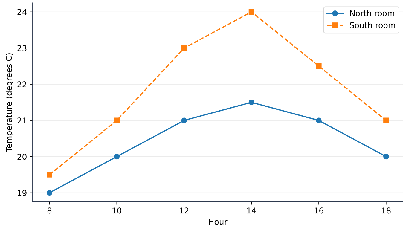
Room temperature comparison
