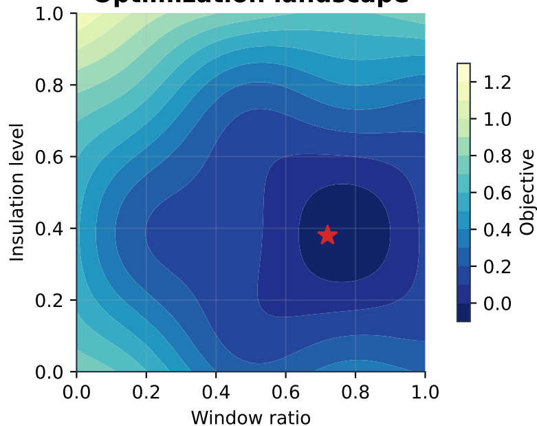
Optimization landscape
