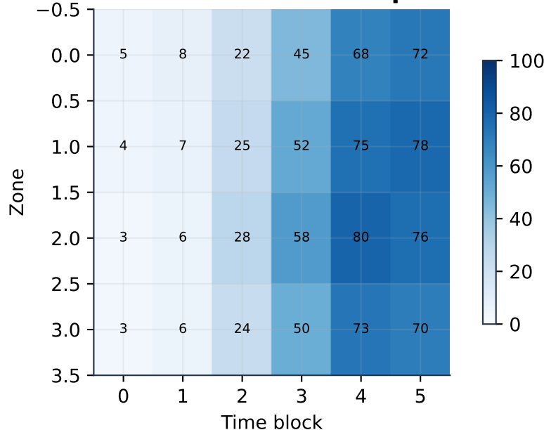
Optimization landscape
