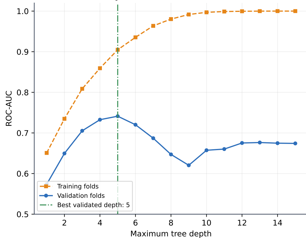
Decision-tree depth versus cross-validated ROC-AUC
