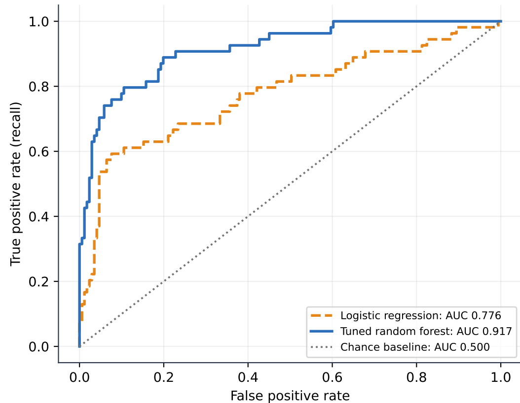
Test-set ROC curves
