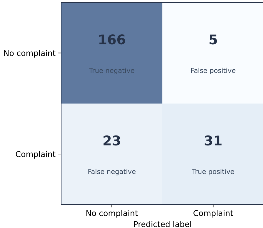
Confusion matrix at threshold 0.50
