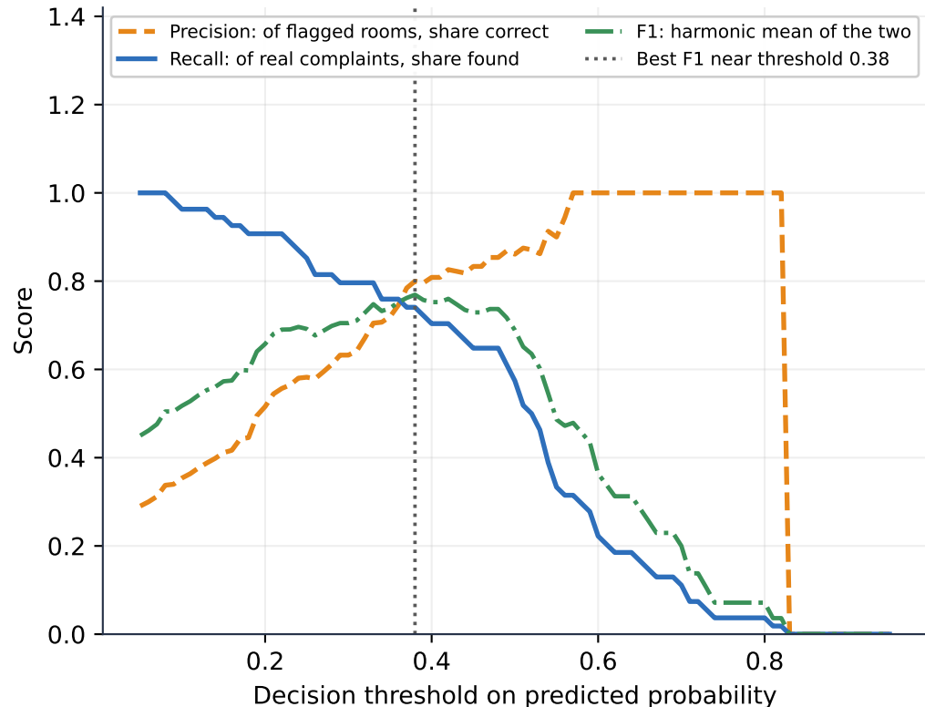
Precision and recall trade off as the threshold moves
