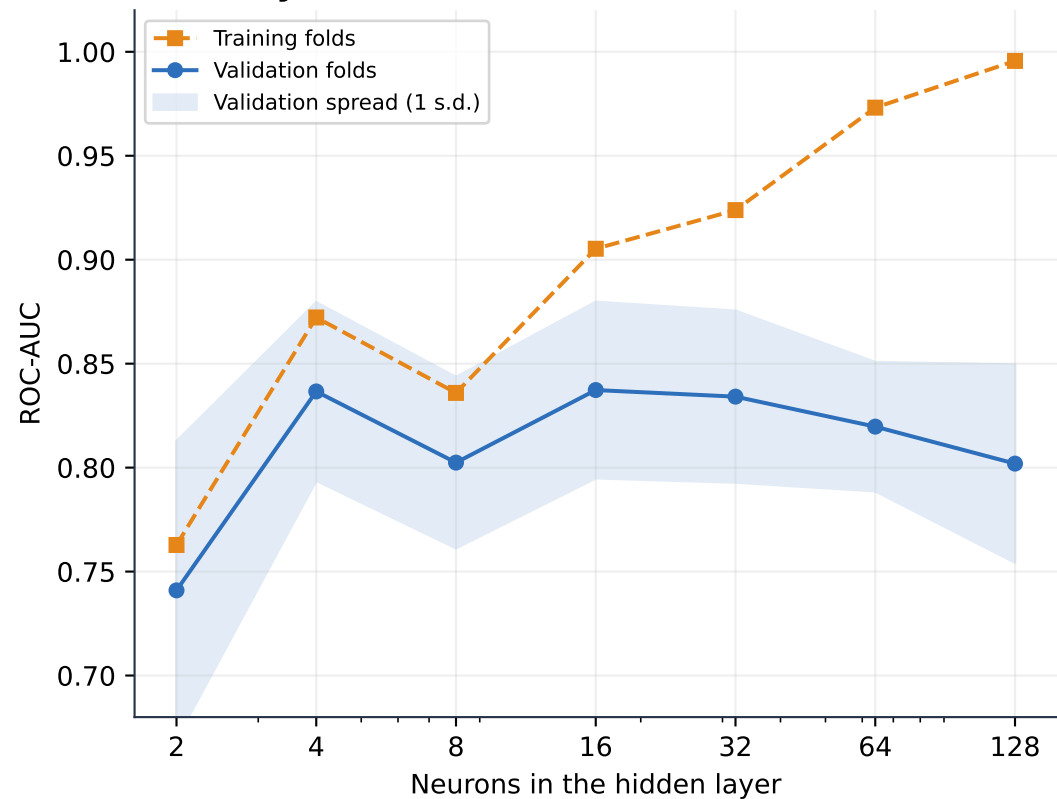
Hidden-layer width versus cross-validated ROC-AUC
