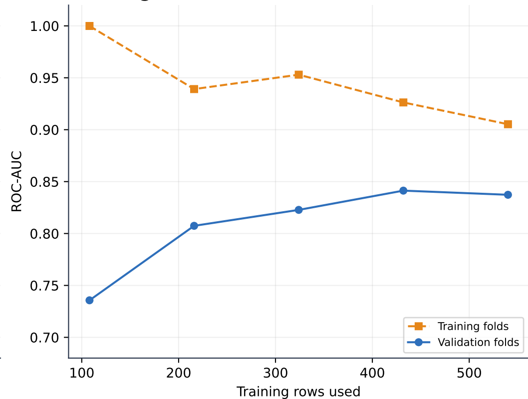
Training rows versus cross-validated ROC-AUC
