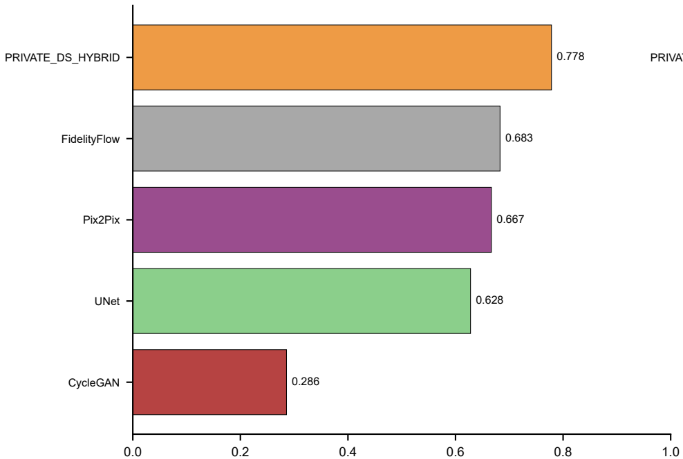
Integrated score
