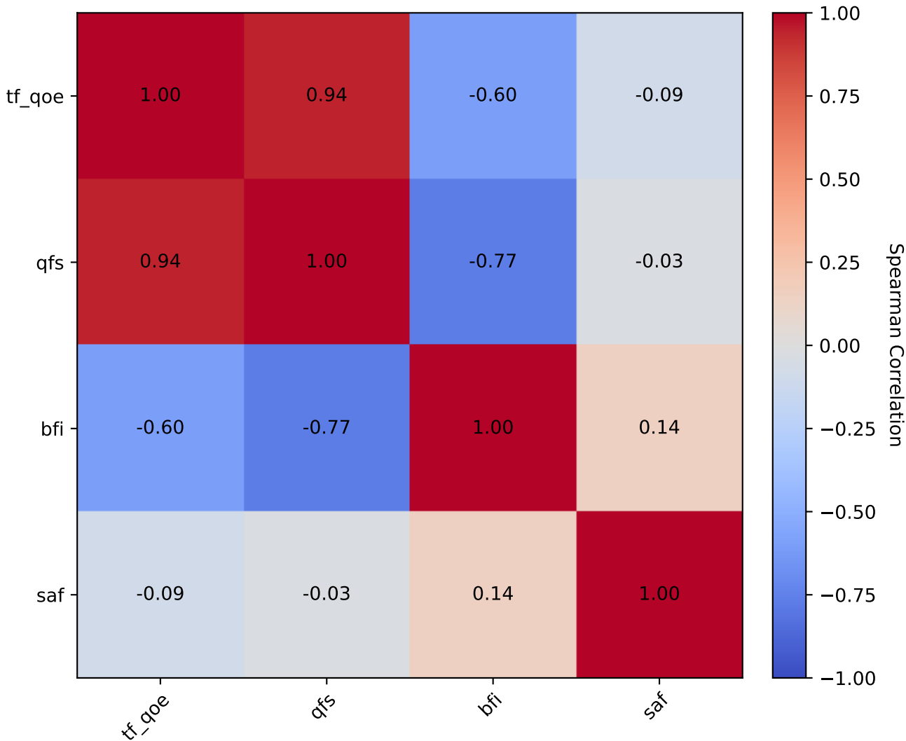
Fairness Metrics
