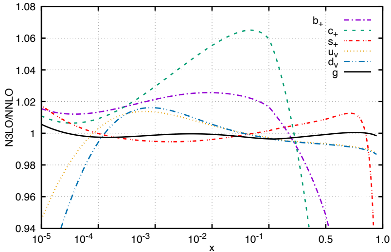
N3LO/NNLO Candia evolution at 100 GeV
