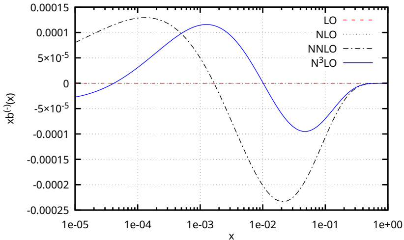
b- PDF using Candia-v2 Evolution at Q=100 GeV
