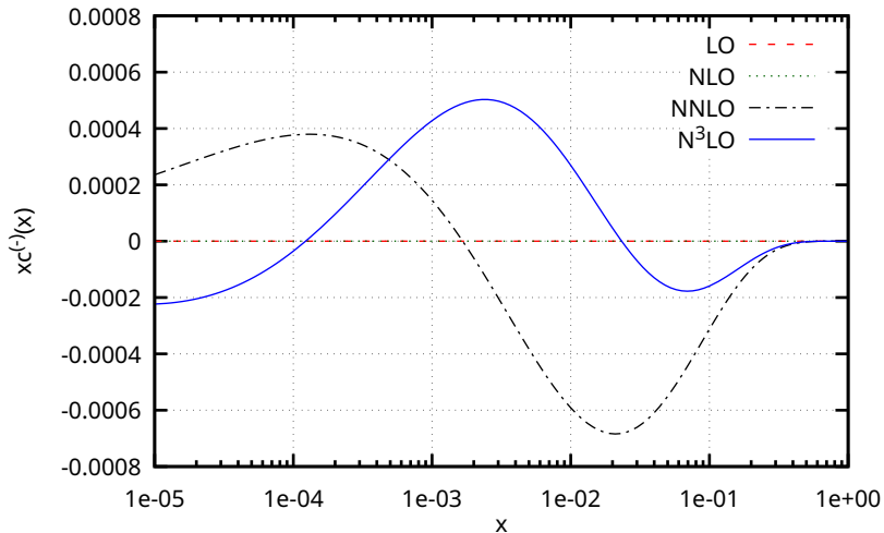
c- PDF using Candia-v2 Evolution at Q=100 GeV
