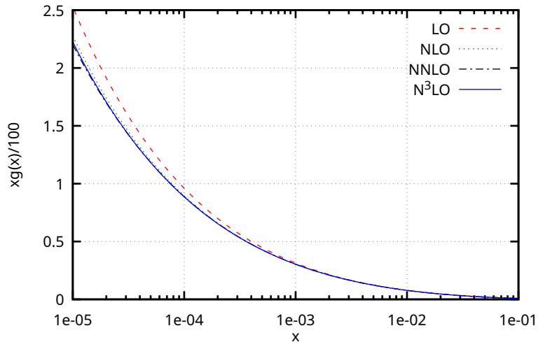
Gluon PDF using Candia-v2 Evolution at Q=100 GeV
