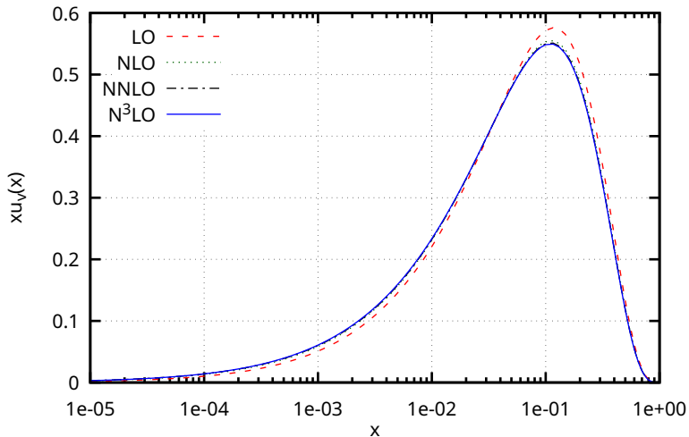
u-valence PDF using Candia-v2 Evolution at Q=100 GeV
