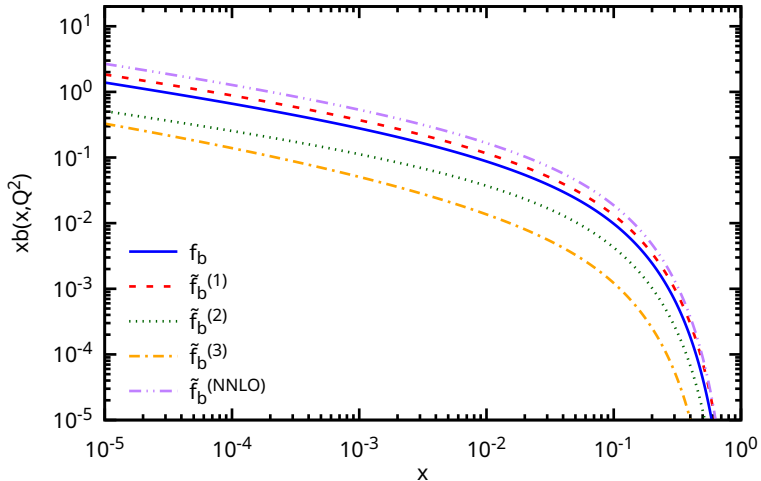
b subtraction PDFs at Q=10 GeV, Candia-v2 evolution
