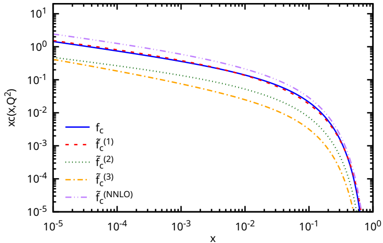
c subtraction PDFs at Q=4 GeV, Candia-v2 evolution
