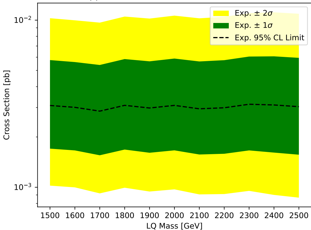
Upper Limit on Cross Section at 95% CL
