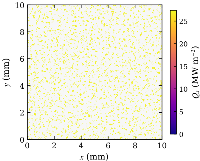
Heat flux at P=10kN
