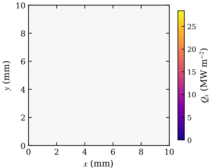
Heat flux at P=50N
