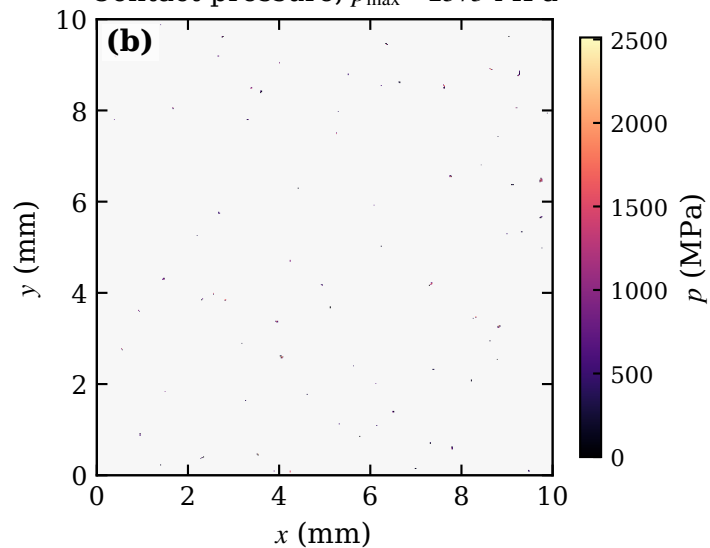
Contact pressure, p_{\max}=2573 MPa
