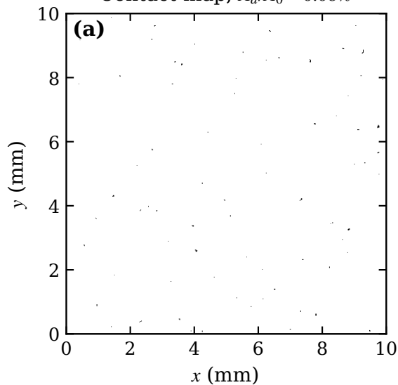
Contact map, A_d/A_0=0.08\%
