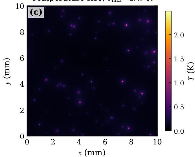
Temperature rise, T_{\max}=2.49 K
