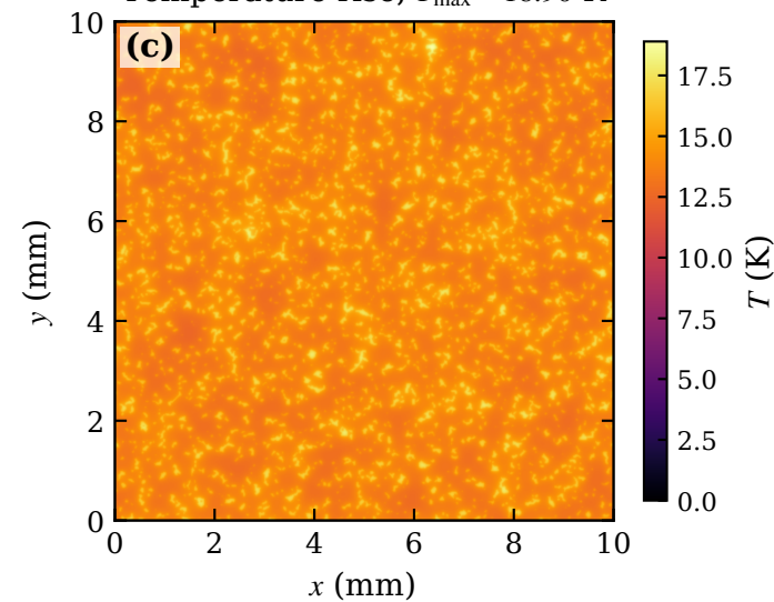
Temperature rise, T_{\max} = 18.90 K
