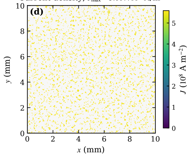
Current density, J_{\max} = 5.60 \times 10^8 A/m 2
