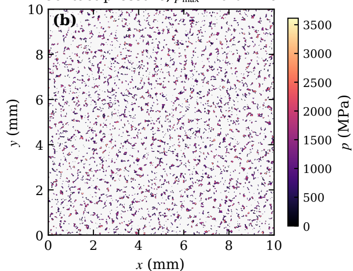
Contact pressure, p_{\max} = 4826 MPa
