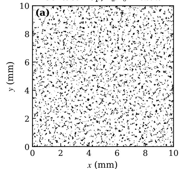
Contact map, A_d/A_0 = 10.39\%
