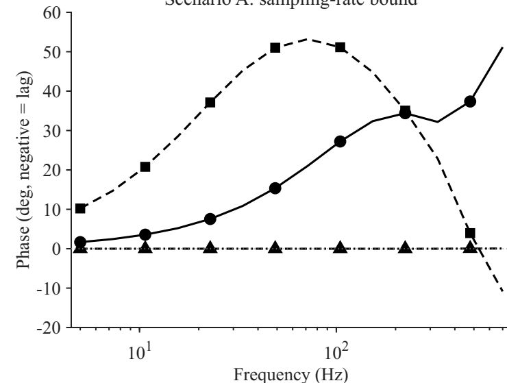
Scenario A: sampling-rate bound
