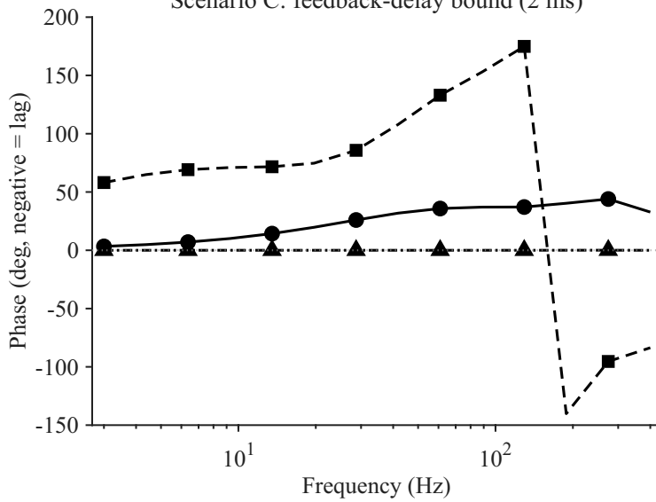
Scenario C: feedback-delay bound (2 ms)
