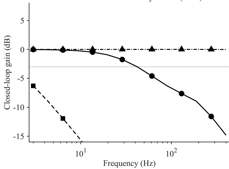
Scenario C: feedback-delay bound (2 ms)
