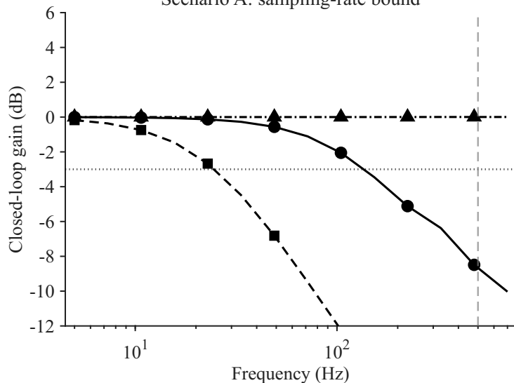
Scenario A: sampling-rate bound
