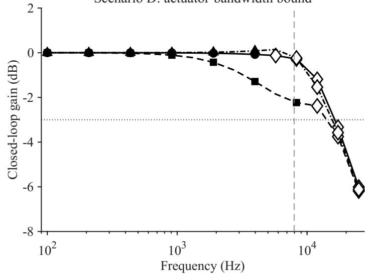
Scenario D: actuator-bandwidth bound
