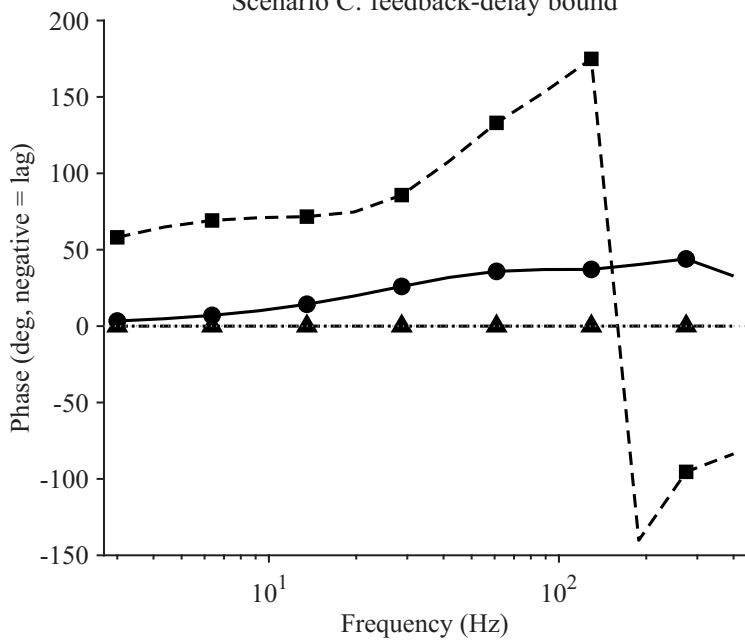
Scenario C: feedback-delay bound
