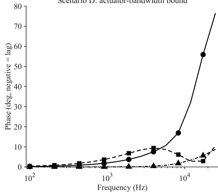
Scenario D: actuator-bandwidth bound
