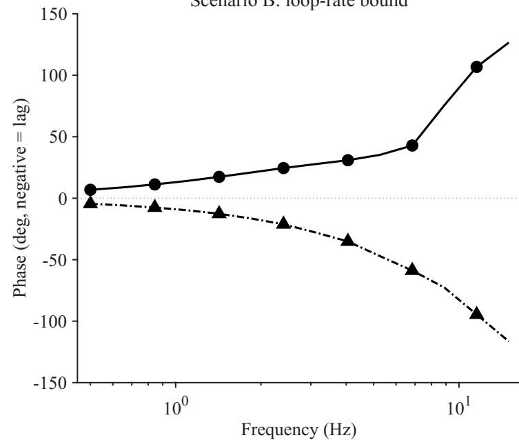
Scenario B: loop-rate bound
