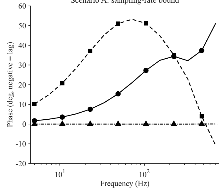
Scenario A: sampling-rate bound
