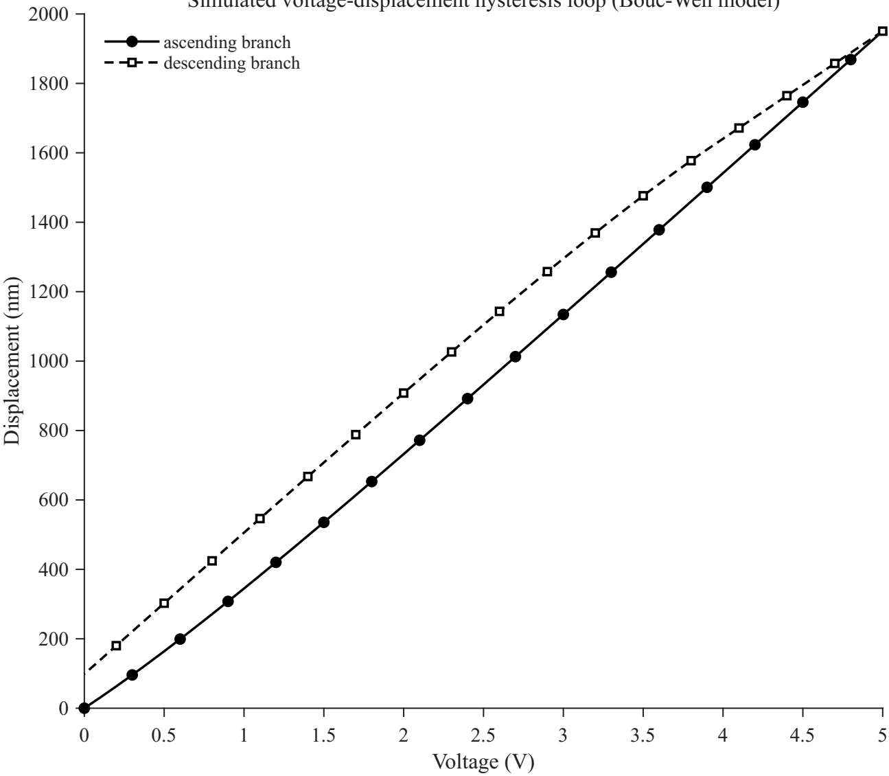
Simulated voltage-displacement hysteresis loop (Bouc-Wen model)
