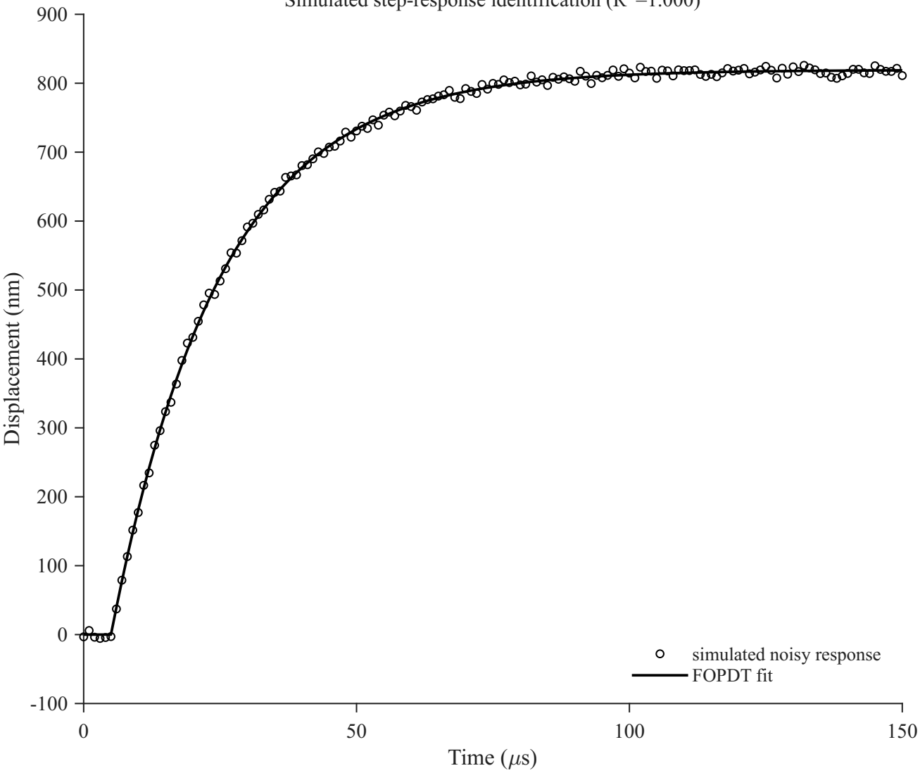
Simulated step-response identification ( R^2=1.000 )
