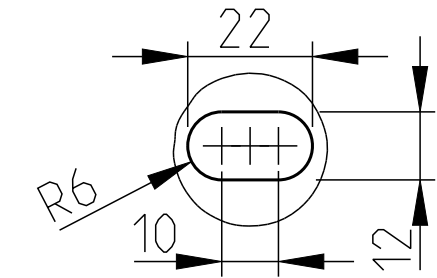
DETAILED VIEW B
