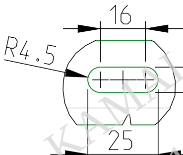
DETAIL VIEW A (2X)
