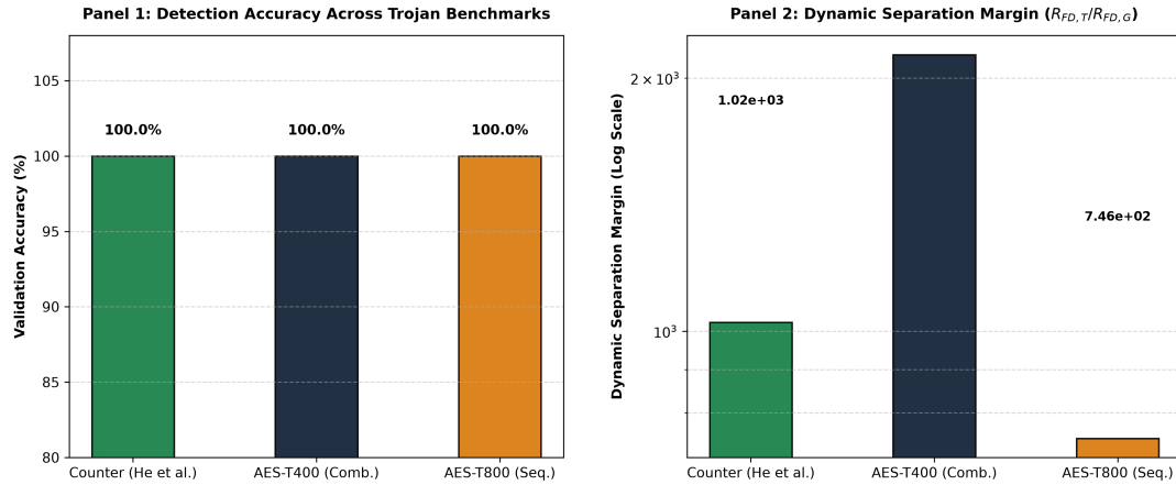
Figure 7.2: Cross-Benchmark Evaluation: (Panel 1) Detection Accuracy Across Trojan Benchmarks; (Panel 2) Dynamic Separation Margin ( R_{FD,T}/R_{FD,G} ) on Log Scale.
