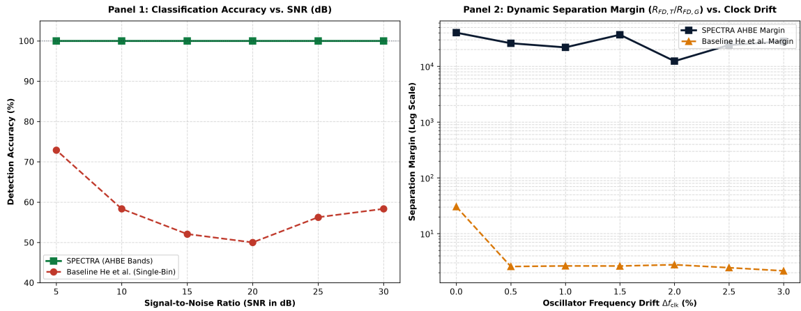
Figure 7.1: Process Variation & SNR Sensitivity Sweep: (Panel 1) Classification Accuracy vs. SNR (dB) comparing Baseline He et al. vs. SPECTRA AHBE; (Panel 2) Dynamic Separation Margin vs. Clock Frequency Drift (%).
