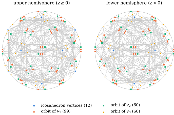
Figure 1: Orthogonal projections of H_{231} onto the xy -plane: vertices with z \geq 0 (left) and z < 0 (right, viewed from below). Marker shape and colour indicate the orbit of G_{372} a vertex belongs to; edges between vertices of the same hemisphere are drawn in grey. The bounding circle has radius r_1 .
