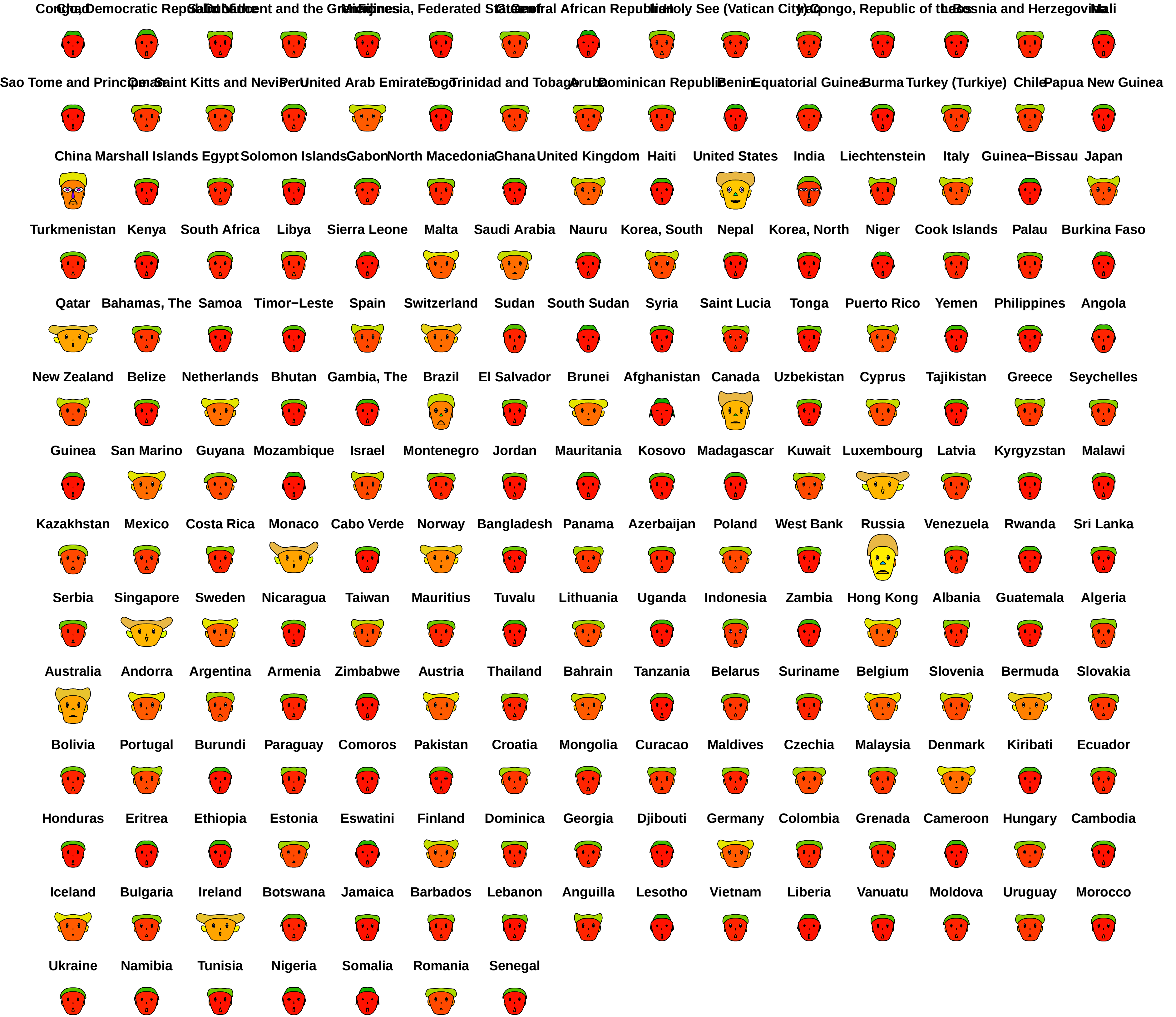
Chernoff Faces of CIA World Factbook Data
