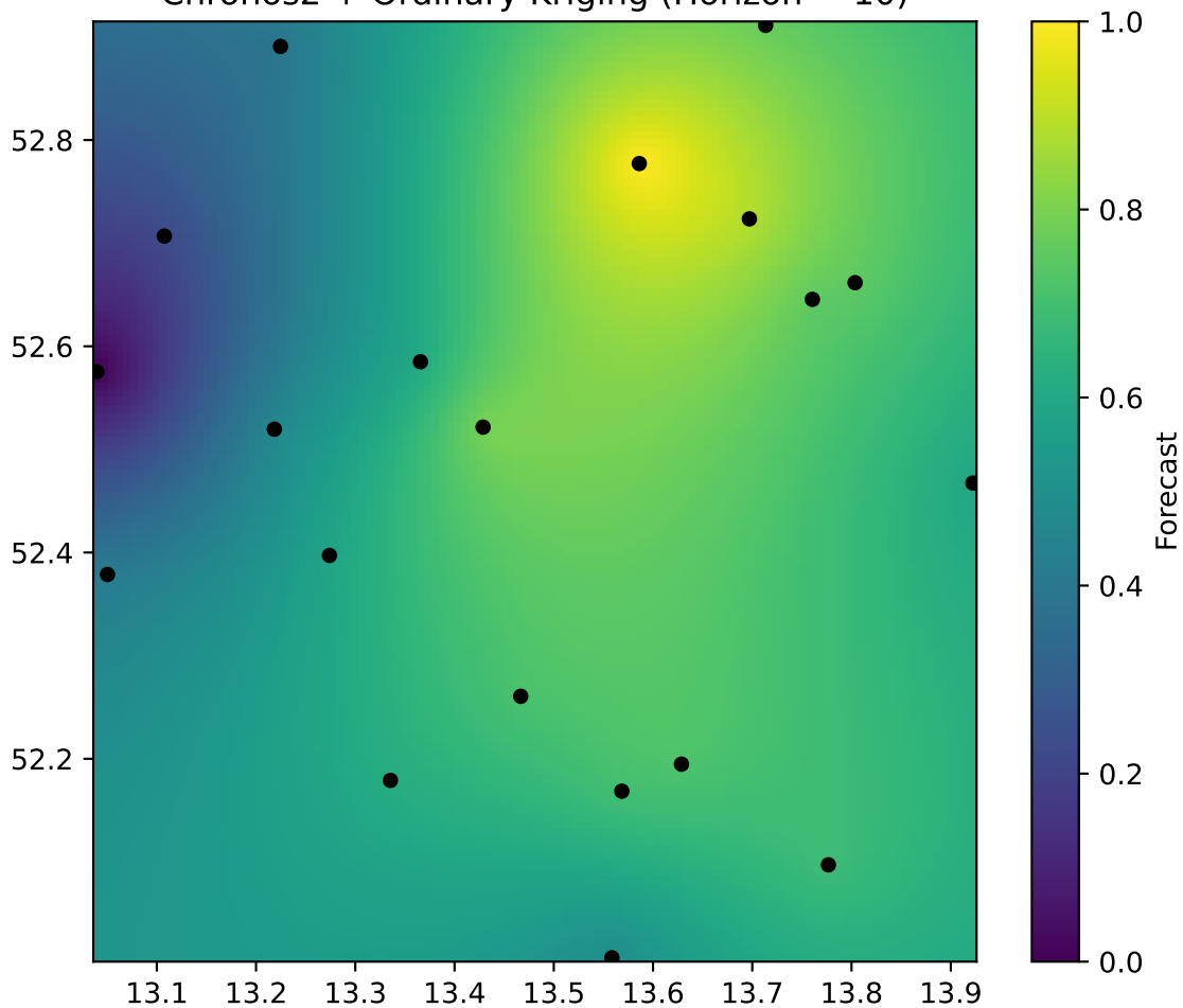
Chronos2 + Ordinary Kriging (Horizon = 10)
