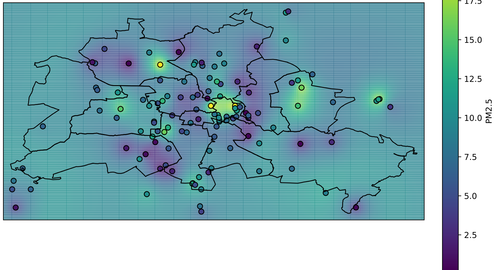
Kriging Heatmap with Berlin Bezirke Overlay
