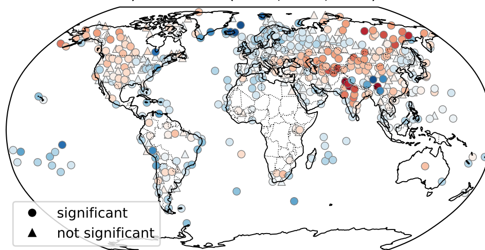
b) IFS-NEMO (-0.07, 0.87, 44%)
