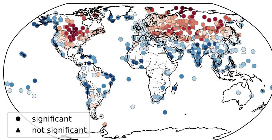
a) ICON (-0.15, 1.89, 43%)
