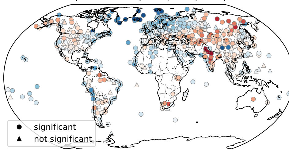
c) IFS-FESOM (-0.17, 0.98, 46%)
