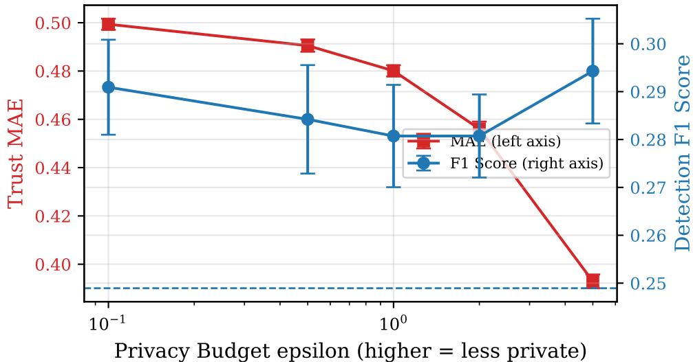
Privacy-Utility Tradeoff (Gaussian DP Mechanism)
