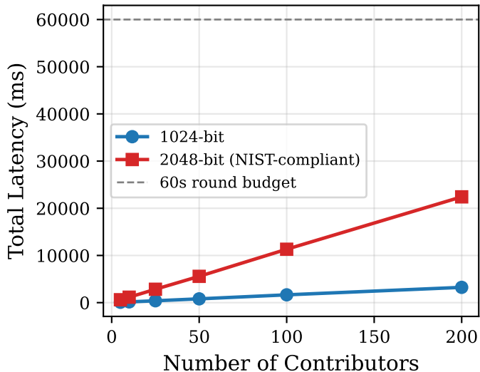
(a) Paillier HE Total Latency
