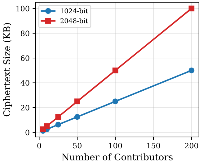
(b) Aggregate Ciphertext Size
