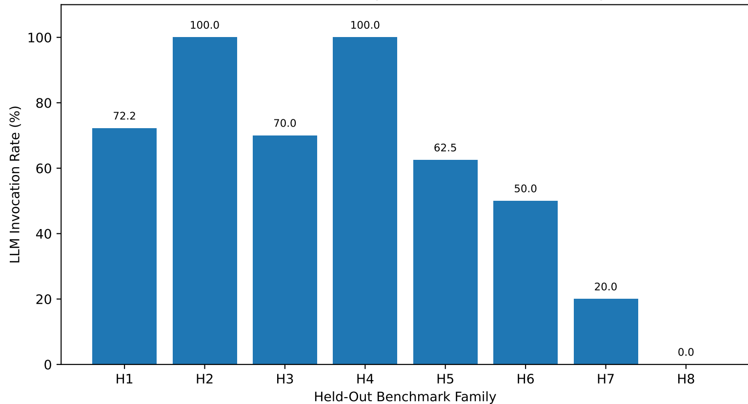
LLM Invocation Rate by Held-Out Benchmark Family
