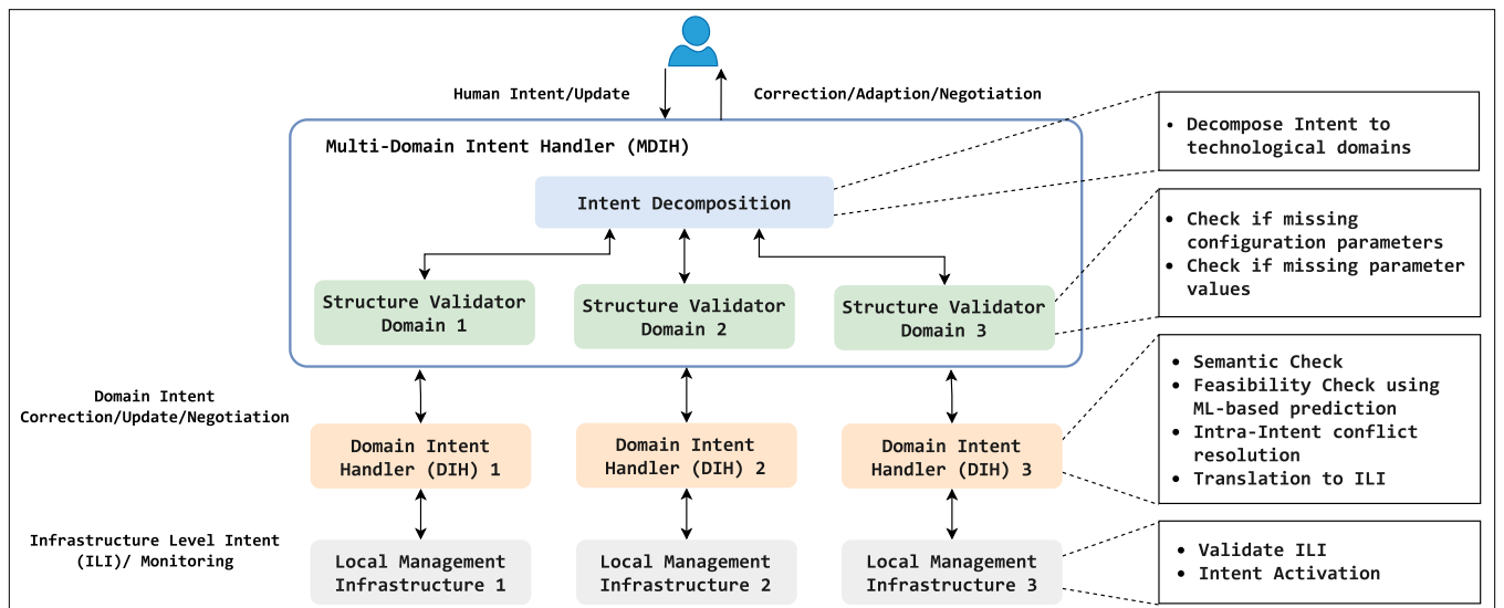
FIGURE 1. High-level architecture design to handle natural language-based Intents LC.
