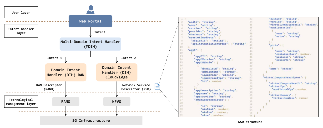
FIGURE 2. Natural language-based Intent LC management in the EURECOM 5G facility [1].
