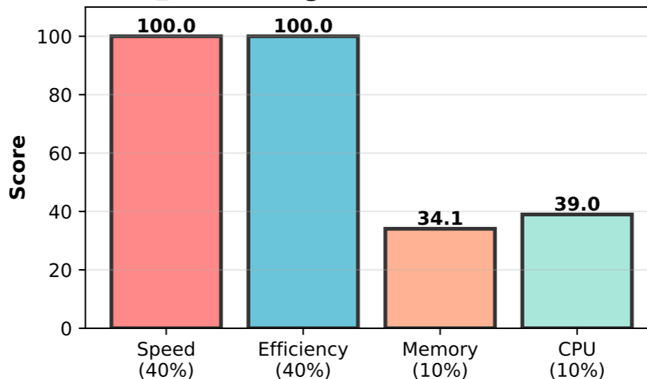
📊 Streaming - Score Breakdown
