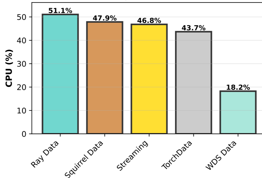
💻 CPU Usage (Lower is Better)
