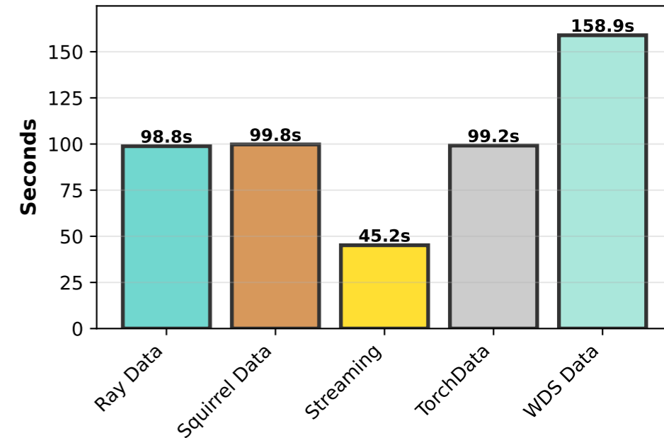
⌚ Processing Time (Lower is Better)
