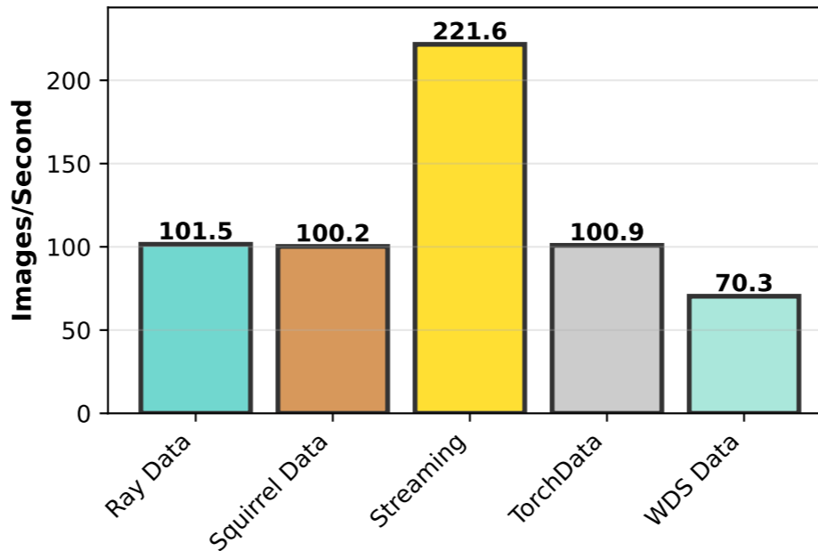
🚀 Throughput (Higher is Better)
