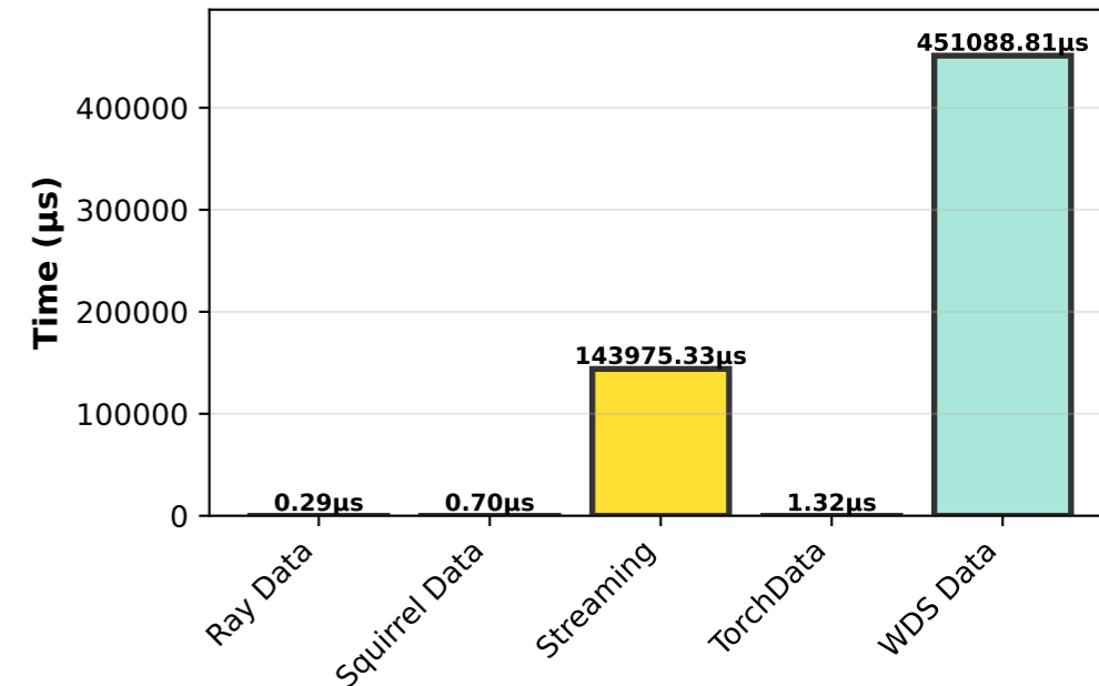
⚙️ Data Load Time (Lower is Better)
