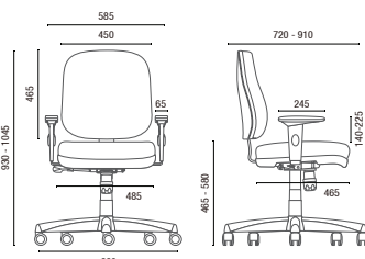
4002 Swivel Midback
