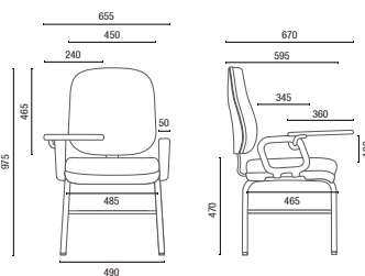
4006 PUE Visitor with Clipboard
