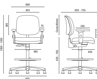
4123 SRE Swivel Stool
