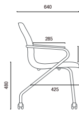
18006 Z ROD Visitor Chair
