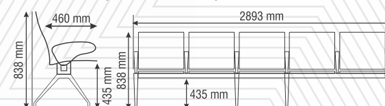
Product No. PLATINUM 5SA 5 Seating (with Armrest)
