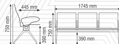
Product No. PELICAN 3SA 3 Seating (with Armrest)
