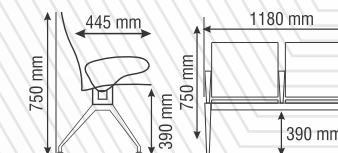
Product No. PELICAN 2SA 2 Seating (with Armrest)
