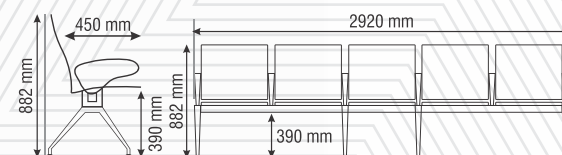
Product No. PRIDE 5SA 5 Seating (with Armrest)
