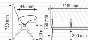
Product No. PELICAN 2S 2 Seating (without Armrest)
