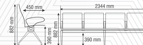
Product No. PRIDE 4SA 4 Seating (with Armrest)
