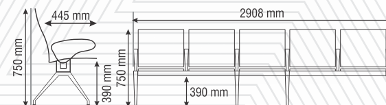
Product No. PELICAN 5SA 5 Seating (with Armrest)
