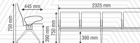
Product No. PELICAN 4SA 4 Seating (with Armrest)
