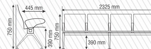
Product No. PELICAN 4S 4 Seating (without Armrest)
