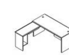
STANDARD TABLE/1.6-7 T160 - 1600W*1700D*750H
