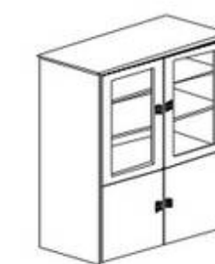
FILLING CABINET WITH 2 GLASS DOOR L80 - 800W * 400D * 2000H
