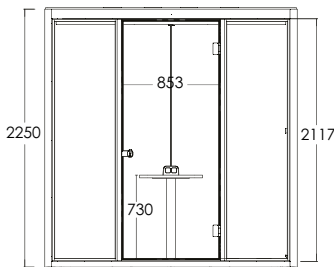
Fixed Center Table
