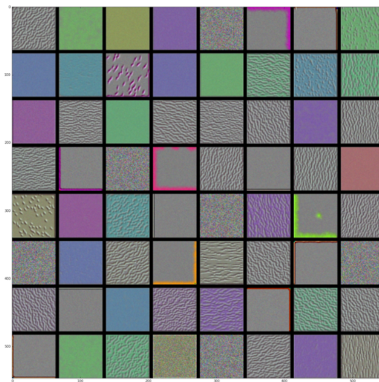
Figure 5.30 Filter patterns for layer block1_conv1
