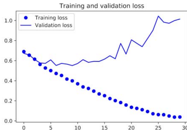
Figure 5.10 Training and validation loss
