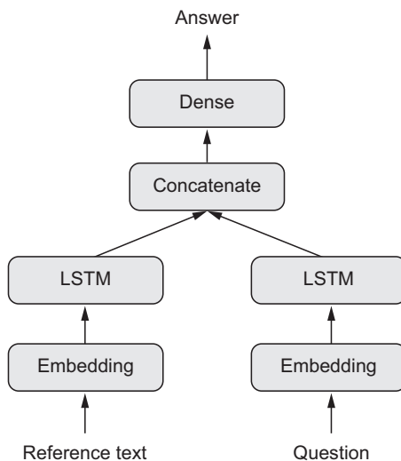
Figure 7.6 A question-answering model
