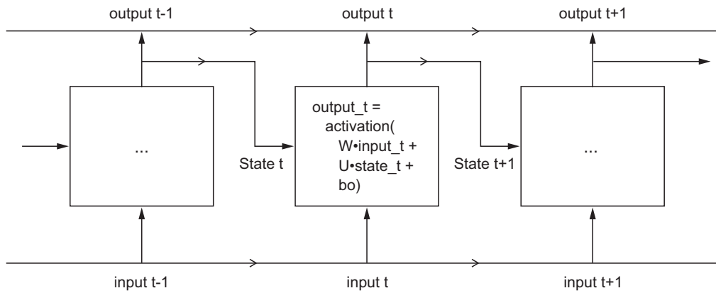
Figure 6.10 A simple RNN, unrolled over time
