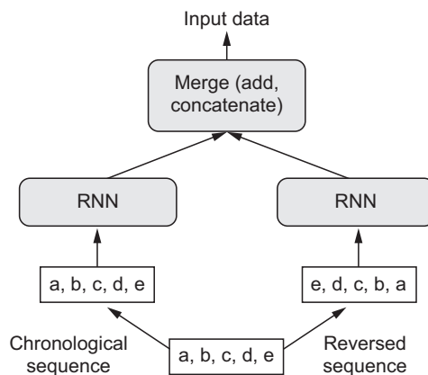
Figure 6.25 How a bidirectional RNN layer works
