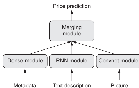
Figure 7.2 A multi-input model
