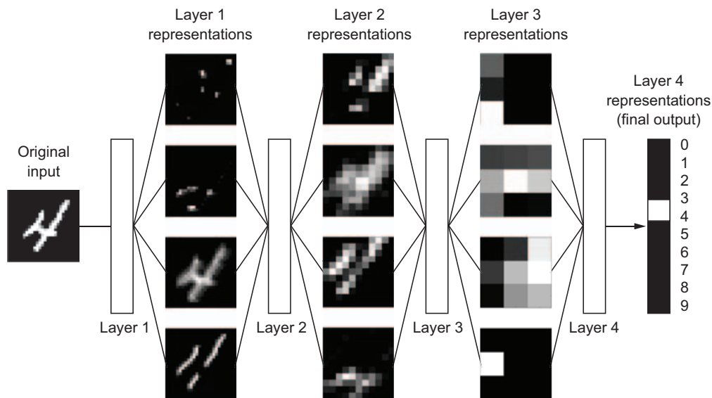
Figure 1.6 Deep representations learned by a digit-classification model
