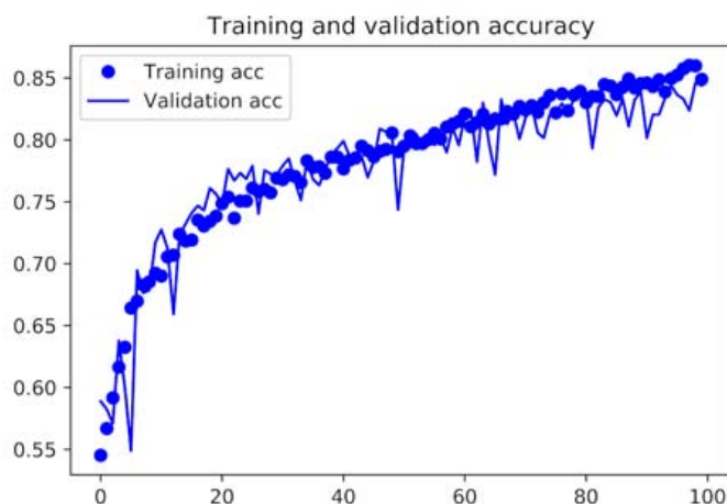
Figure 5.12 Training and validation accuracy with data augmentation
