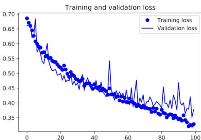
Figure 5.13 Training and validation loss with data augmentation
