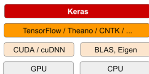
Figure 3.3 The deep-learning software and hardware stack
