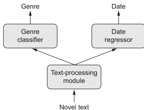
Figure 7.3 A multi-output (or multihead) model
