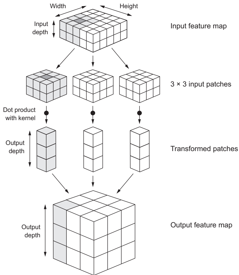
Figure 5.4 How convolution works
