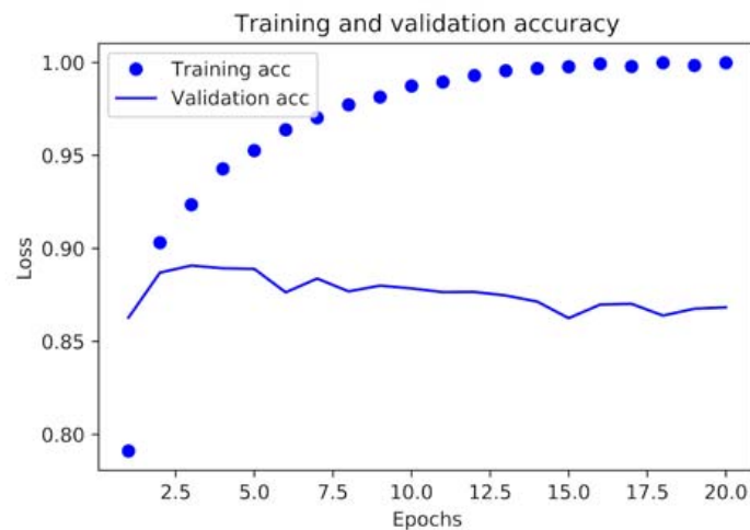
Figure 3.8 Training and validation accuracy
