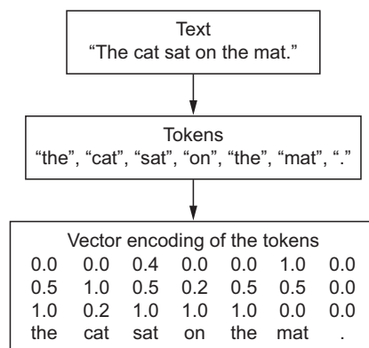
Figure 6.1 From text to tokens to vectors
