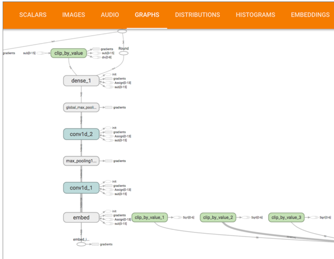
Figure 7.13 TensorBoard: TensorFlow graph visualization
