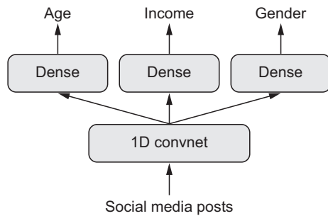
Figure 7.7 A social media model with three heads
