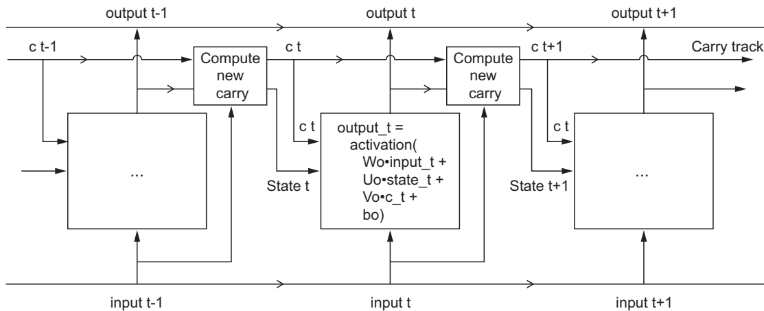
Figure 6.15 Anatomy of an LSTM
