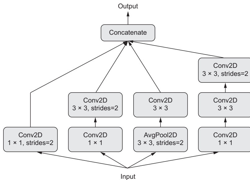
Figure 7.8 An Inception module
