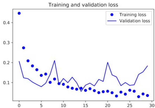
Figure 5.21 Training and validation loss for fine-tuning
