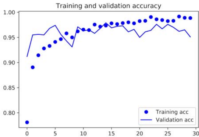
Figure 5.20 Training and validation accuracy for fine-tuning
