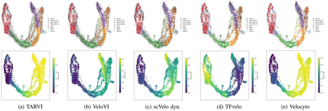
Fig. 3: Pancreas UMAP (same column order in both rows). Top: velocity streamlines; cells coloured by annotated cell type, arrows depict the projected RNA velocity field. Bottom: inferred latent time (early to late).
