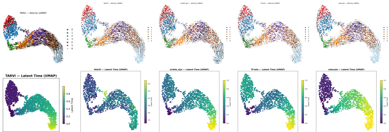
Figure S2: Forebrain (UMAP): velocity streamlines (top) and inferred latent time (bottom) for each method; panels are titled by method.
