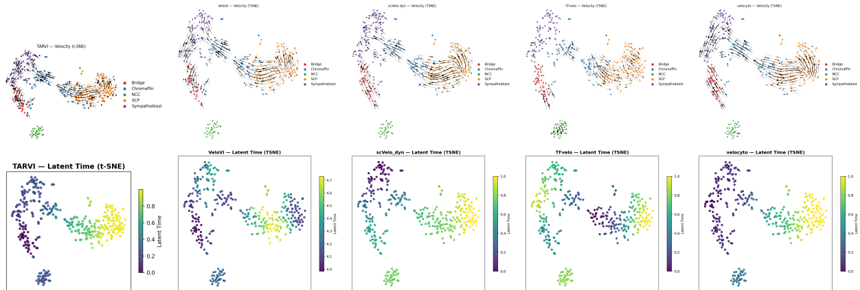
Figure S1: Chromaffin (t-SNE): velocity streamlines (top) and inferred latent time (bottom) for each method; panels are titled by method.
