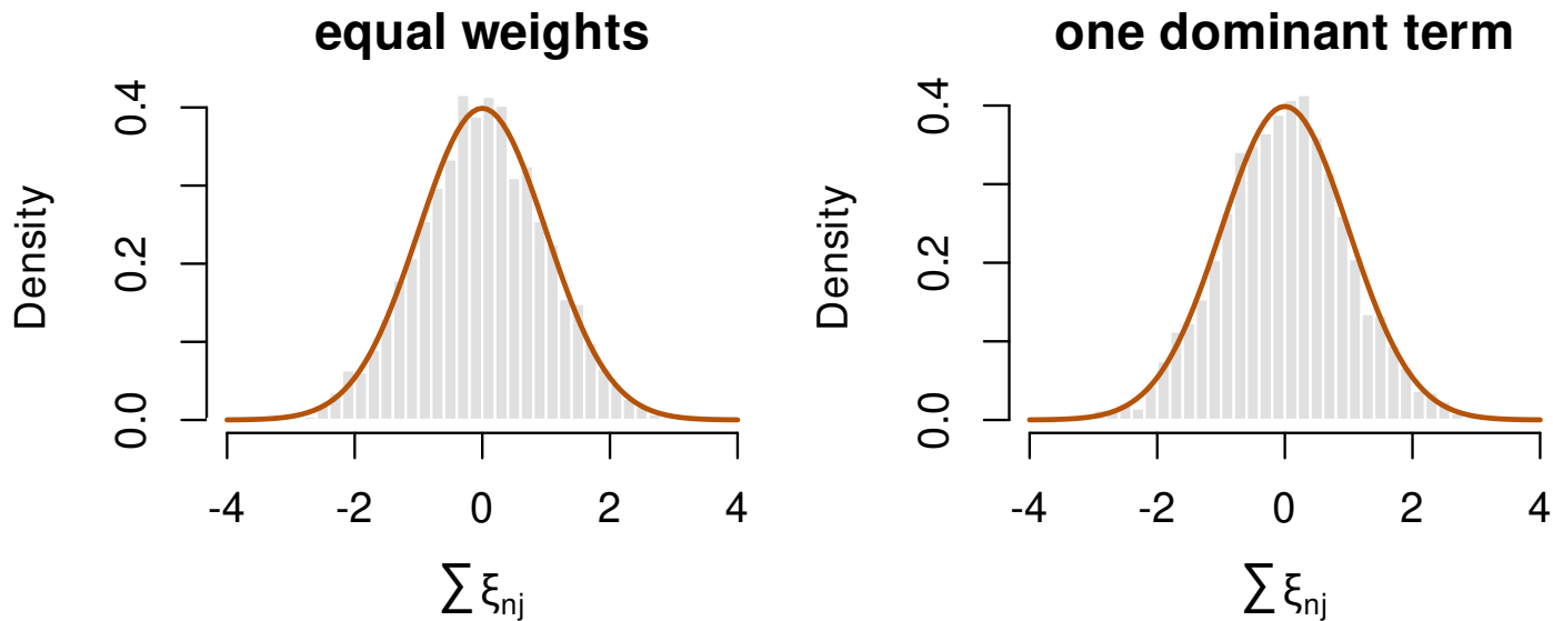
Figure P.1: Row sums of a triangular array against the N(0, 1) density. Both rows have total variance 1; only the left satisfies (P.22). In the right panel the sum is a sum of two normals and so is itself exactly normal. The illustration is that the limit is not reached by accumulation , the dominant term never becoming negligible.
